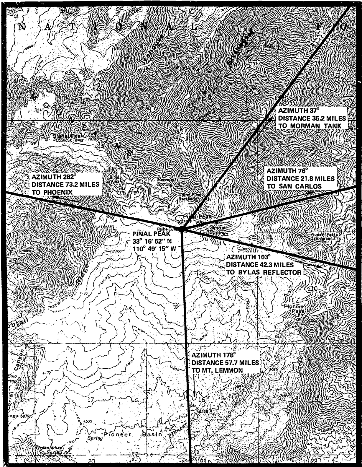
Figure B.9. Pinal Peak Site Map.
