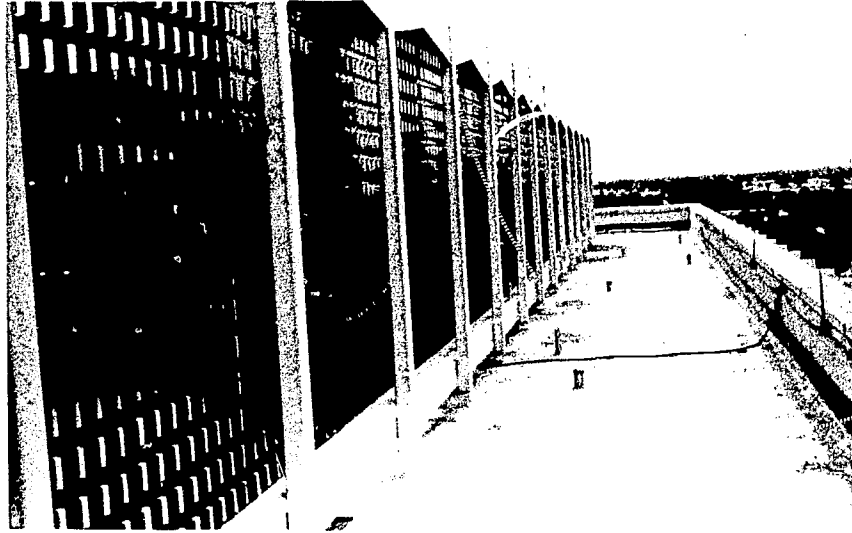
Figure C-45. Phoenix Indian Medical Center Roof Showing Lightning Rod Ground System and Grillwork Surrounding the Penthouse.
