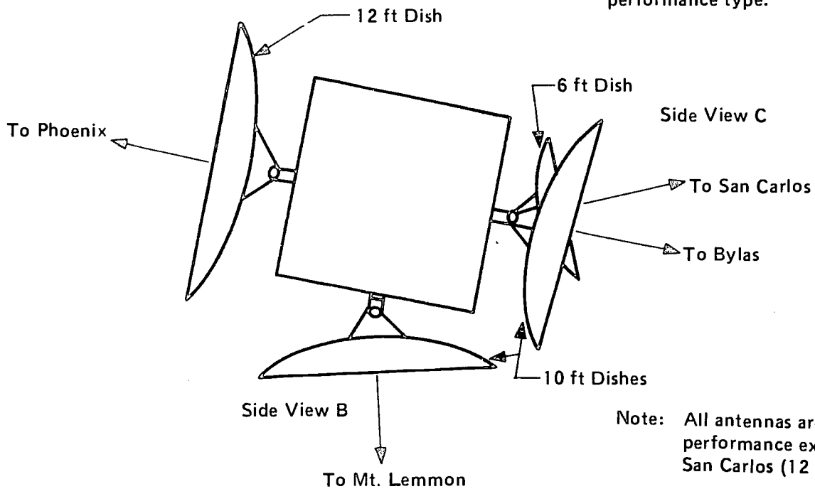
Figure D.55. New Tower and Antenna Arrangement at Pinal Peak.
