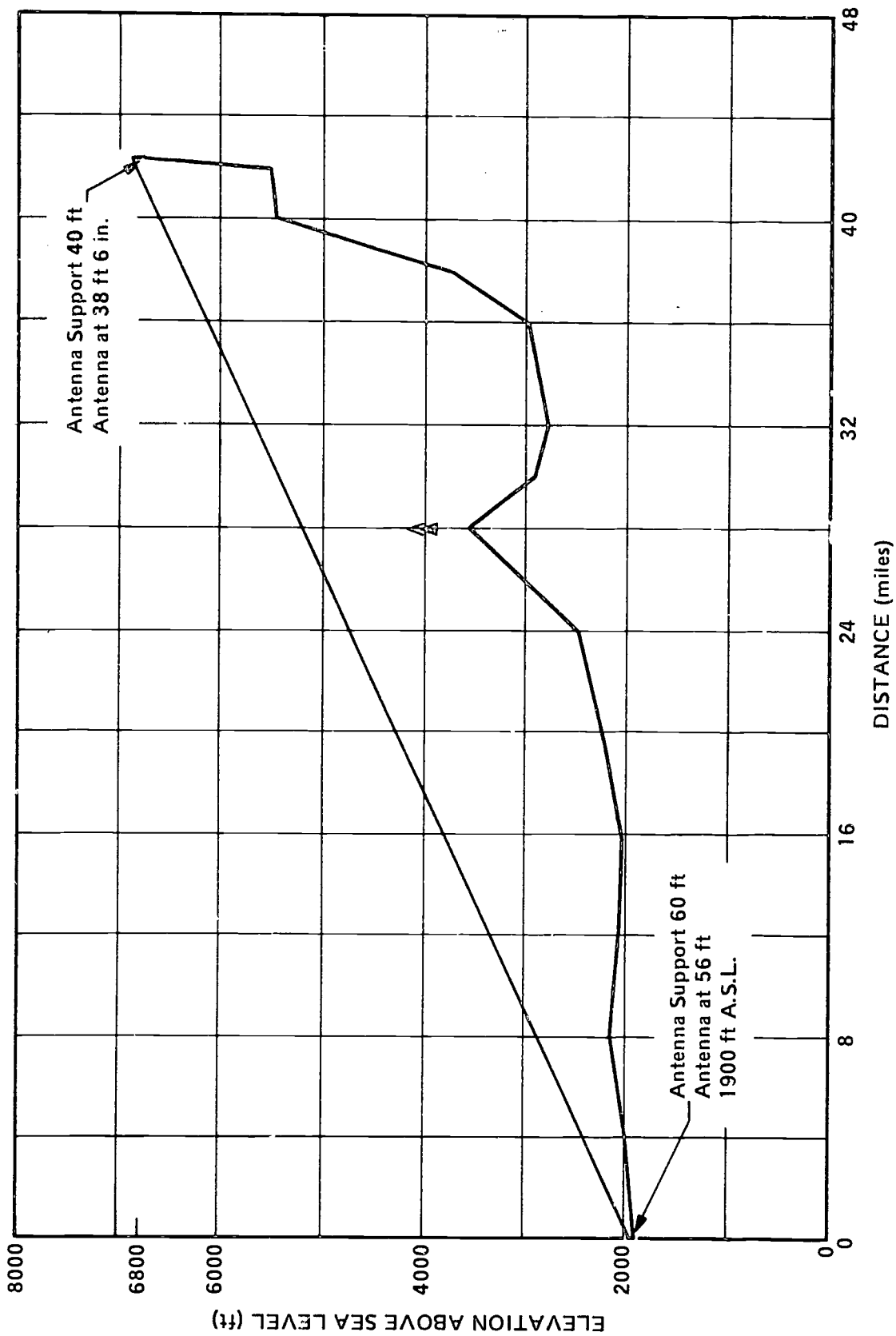
Figure A.2. Microwave Path Profile, Pisanimo to Kitt Peak.
