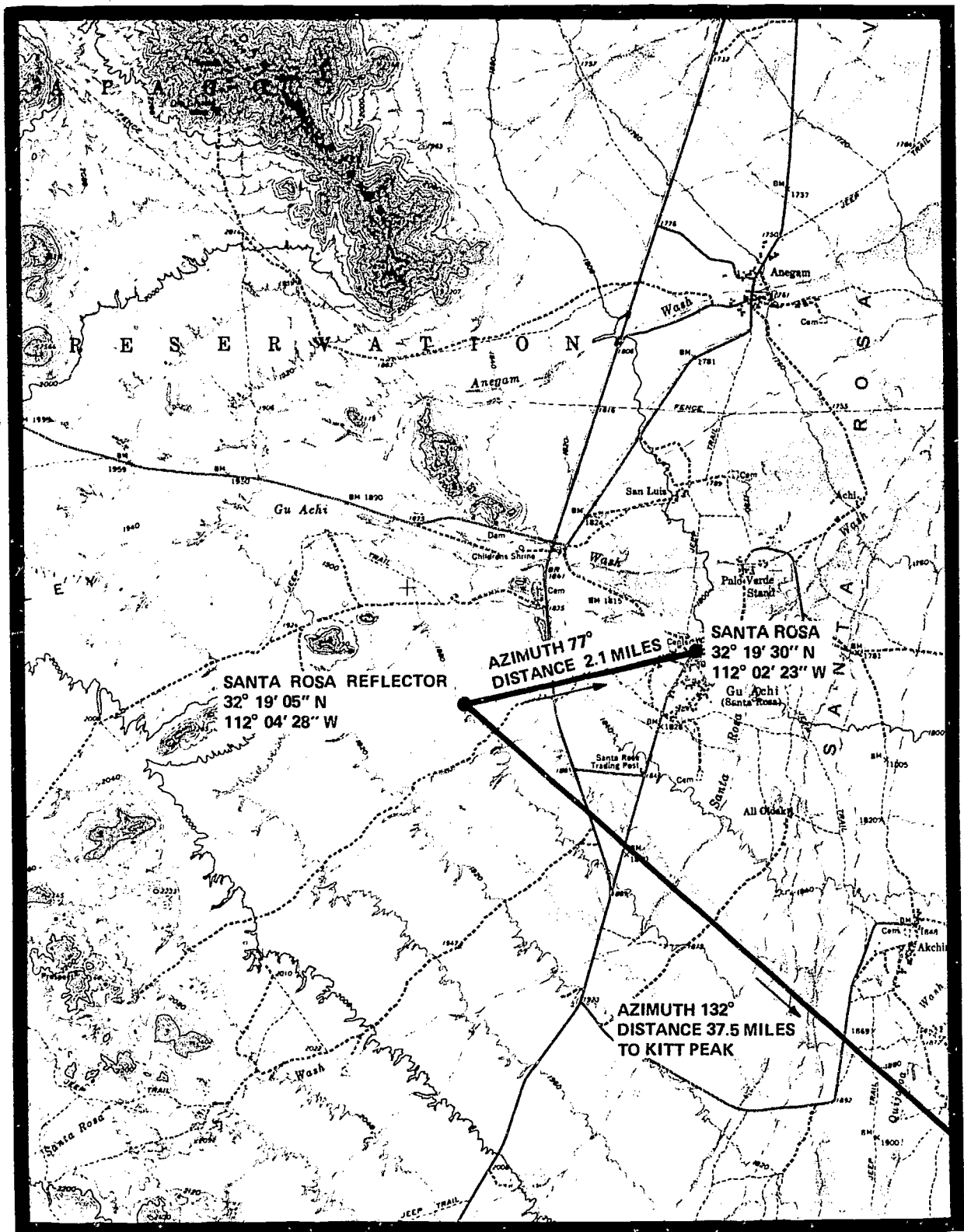
Figure B.4. Santa Rosa Site Map.
